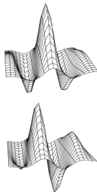
Gabor Wavelets
